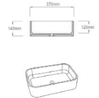
Side cross-section
