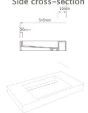
Side cross-section
